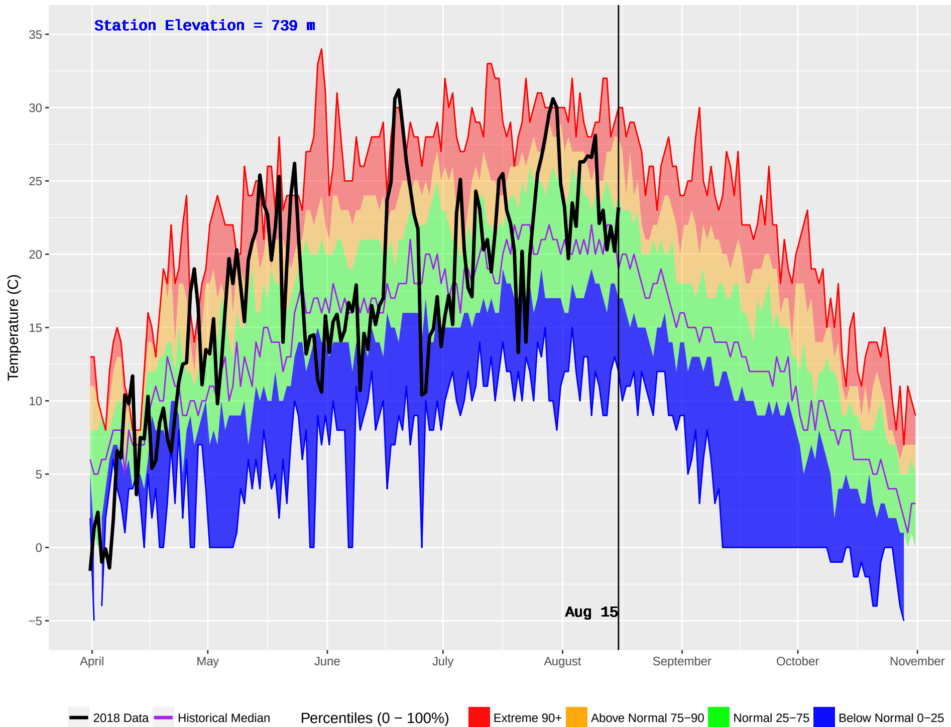
BEAR LAKE (149) : Historical (1980–2016) and Current (2018) Daily Temperature
