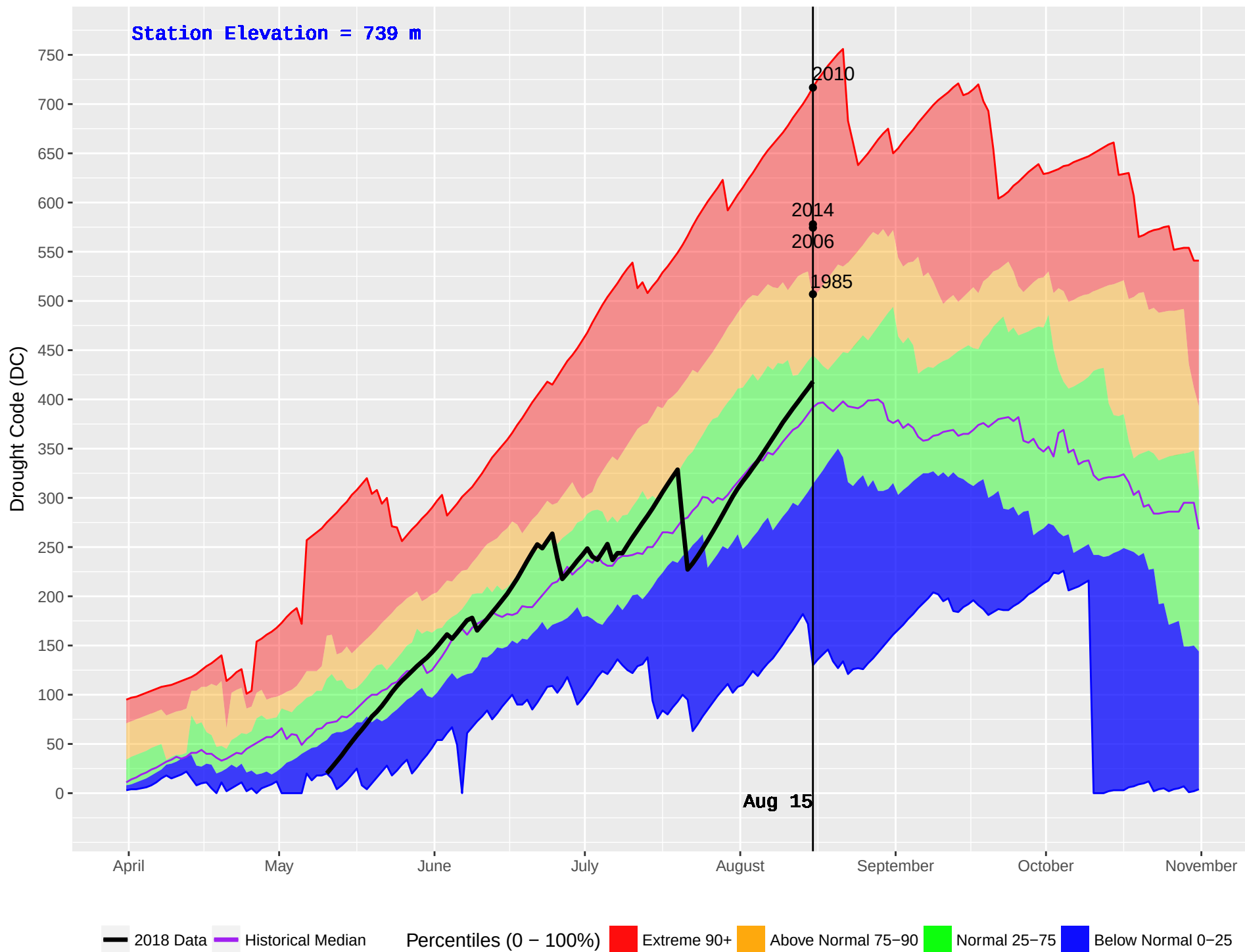
BEAR LAKE (149) : Historical (1980–2016) and Current (2018) Daily Drought Code (DC)
