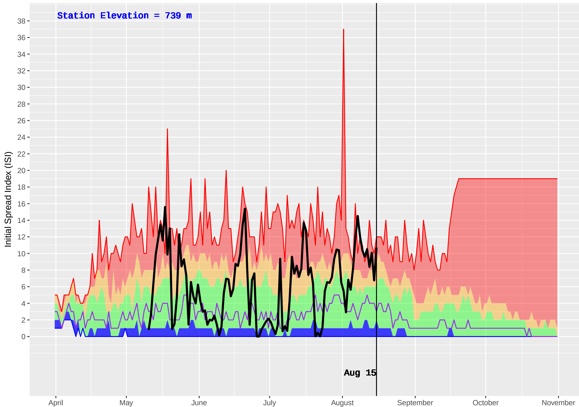
BEAR LAKE (149) : Historical (1980–2016) and Current (2018) Daily Initial Spread Index (ISI)
