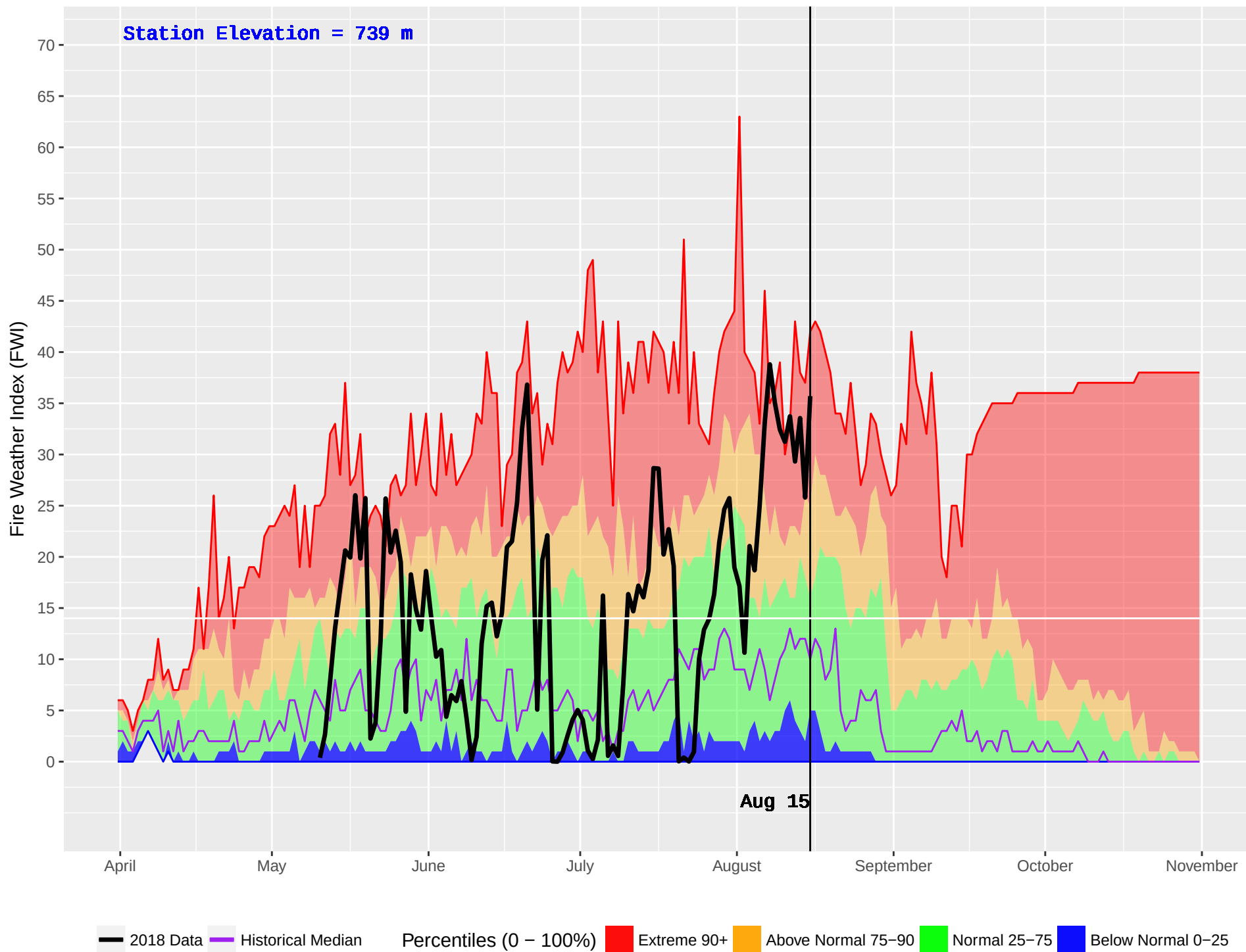
BEAR LAKE (149) : Historical (1980–2016) and Current (2018) Daily Fire Weather Index (FWI)
