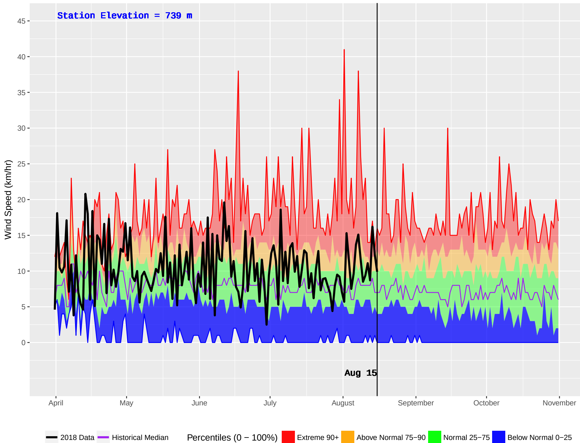
BEAR LAKE (149) : Historical (1980–2016) and Current (2018) Daily Wind Speed
