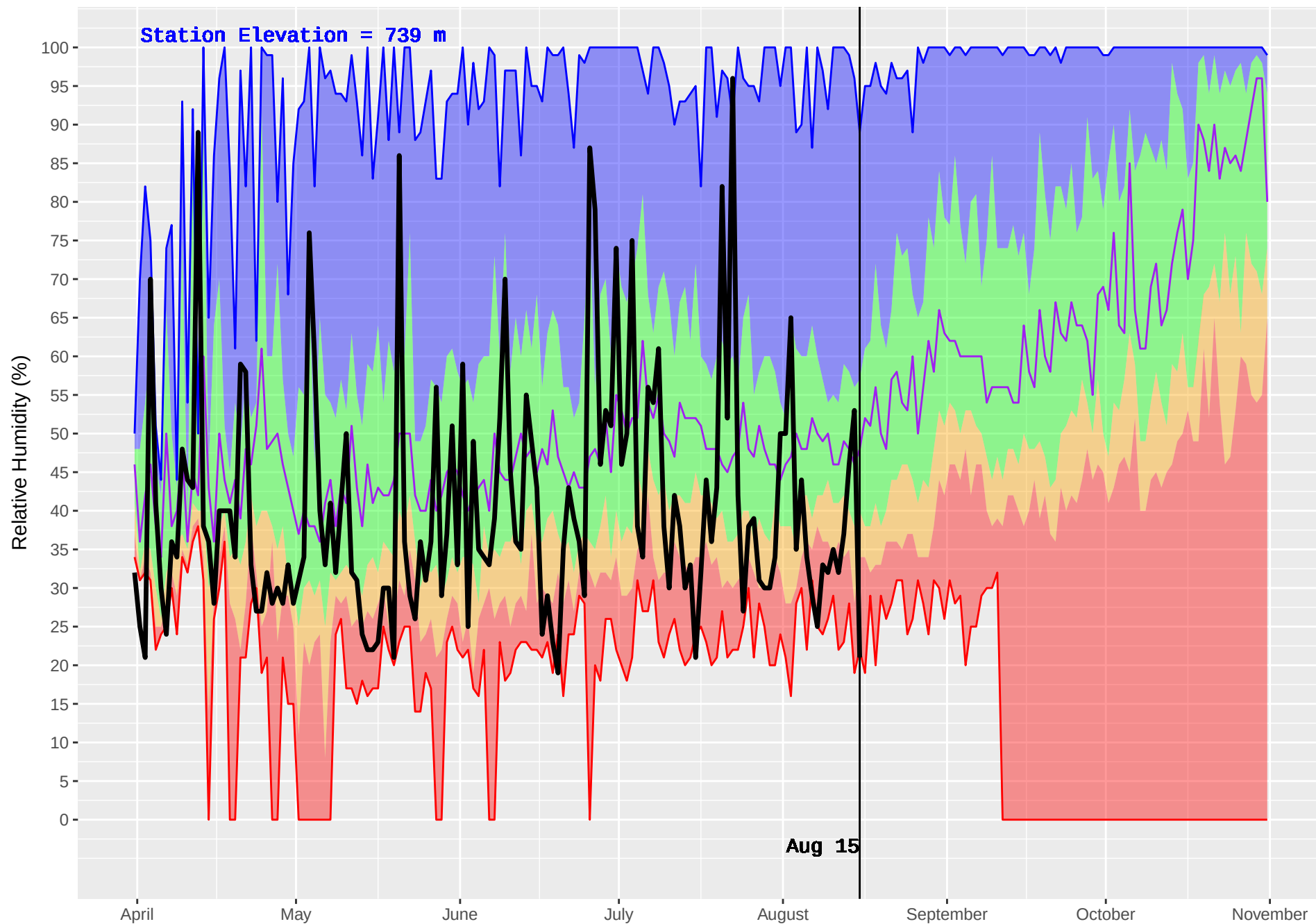
BEAR LAKE (149) : Historical (1980–2016) and Current (2018) Daily Relative Humidity
