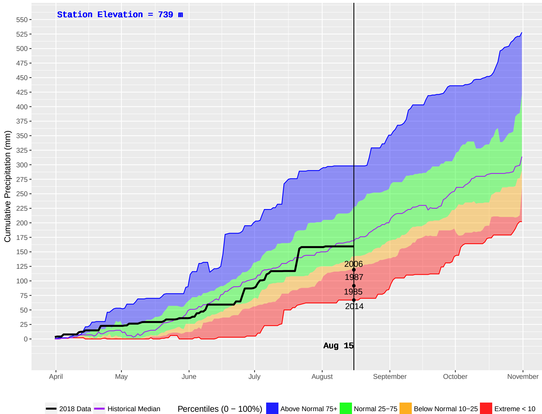
BEAR LAKE (149) : Historical (1980–2016) and Current (2018) Daily Cumulative Precipitation
