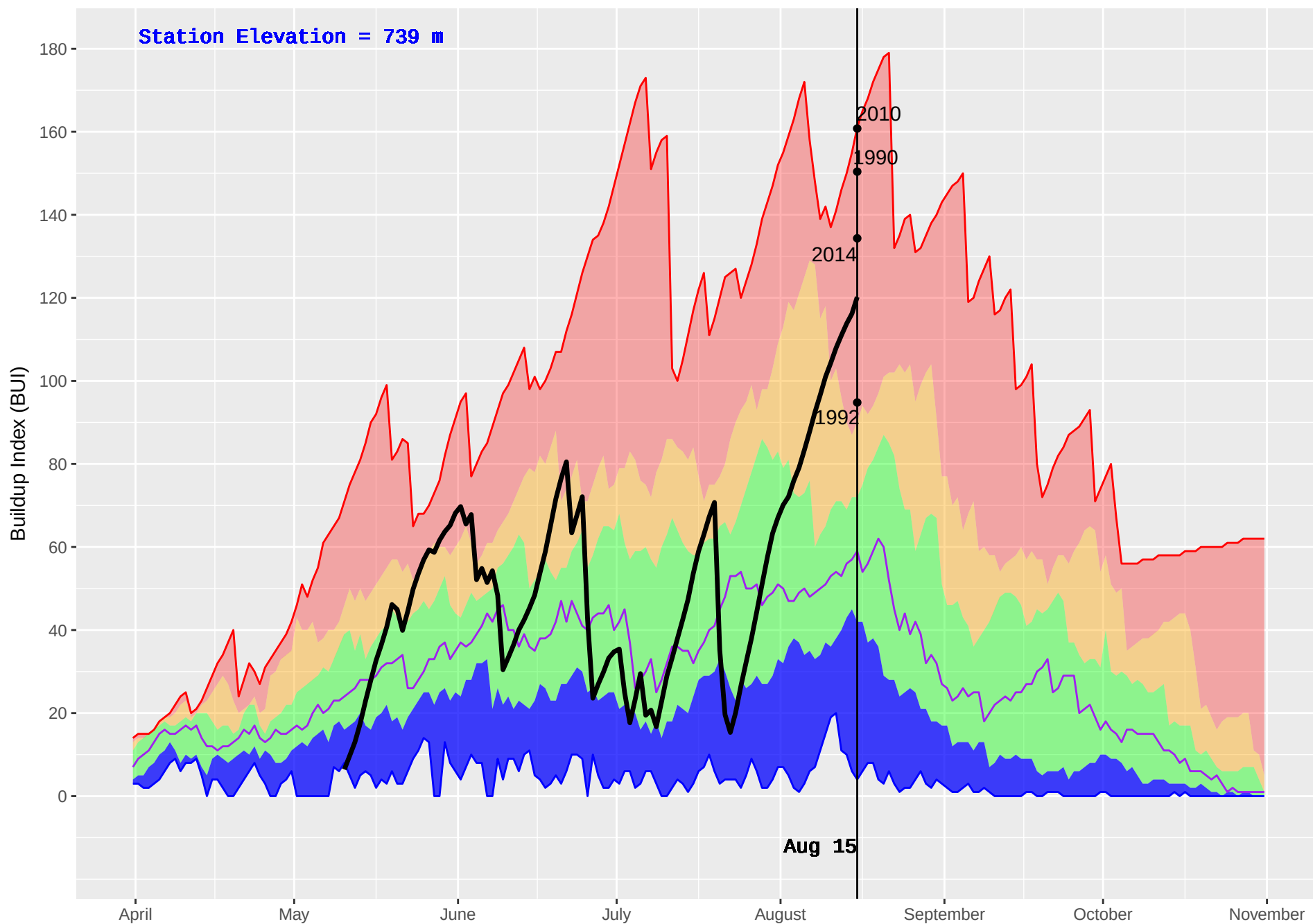
BEAR LAKE (149) : Historical (1980–2016) and Current (2018) Daily Buildup Index (BUI)
